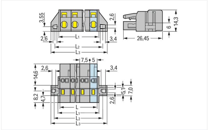
Dimensions in mm L = (pole no. – 1) x pin spacing + 5 mm L1 = L + 3 mm L2 = L + 8.8 mm L3 = L + 14.8 mm 2- to 3-pole female connectors – one latch only
