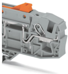
Cover (2006-191) seals unused conductor entry.
