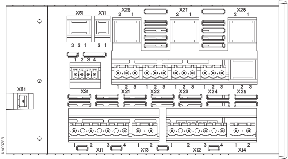
Figure 5.3 Connectors, OMD200
