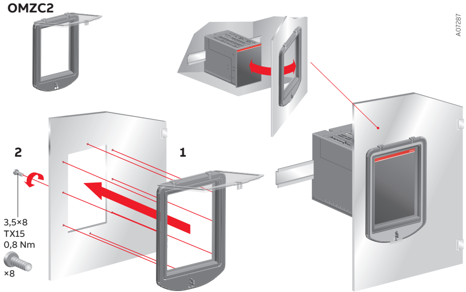
Figure 4.5 Automatic control unit OMD_, DIN-rail mounting with the cover plate, door drilling for the cover plate OMZC2, see Accessories, Section 10
