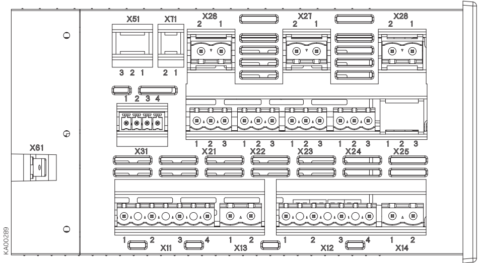
Figure 5.6 Connectors, OMD300
