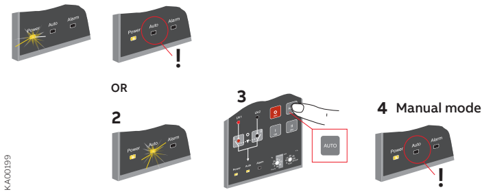
Figure 6.7 Selecting the automatic control units OMD200 and OMD300 to Manual Mode
