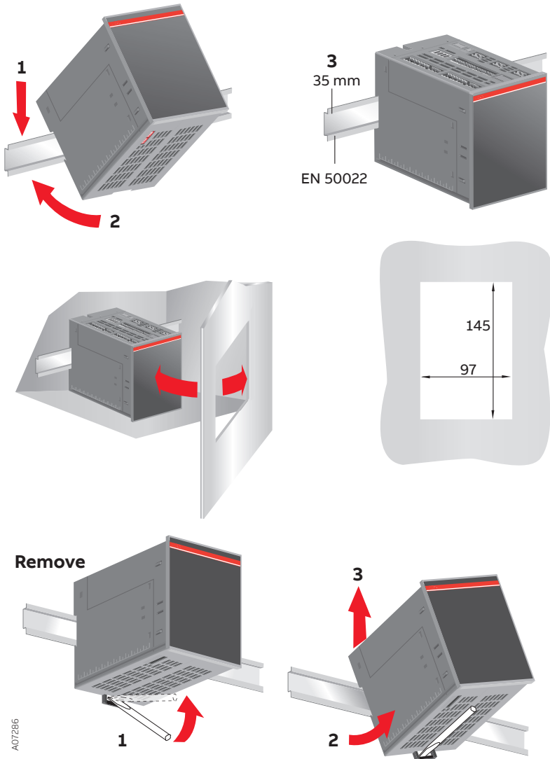
Figure 4.4 Automatic control unit OMD_, DIN-rail mounting, door drilling
