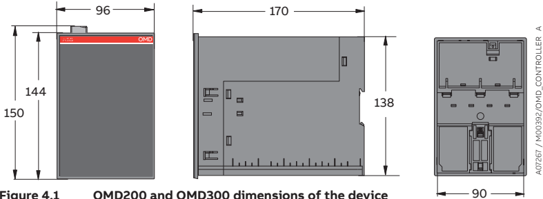
Figure 4.1 OMD200 and OMD300 dimensions of the device
