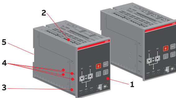
Figure 2.1 Automatic control units, OMD200 and OMD300
