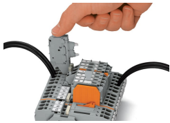
Fused disconnect terminal block with a pivoting fuse holder Pivot the fuse holder into the locked open position.
