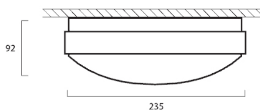
Giotto 235 surface mounted
