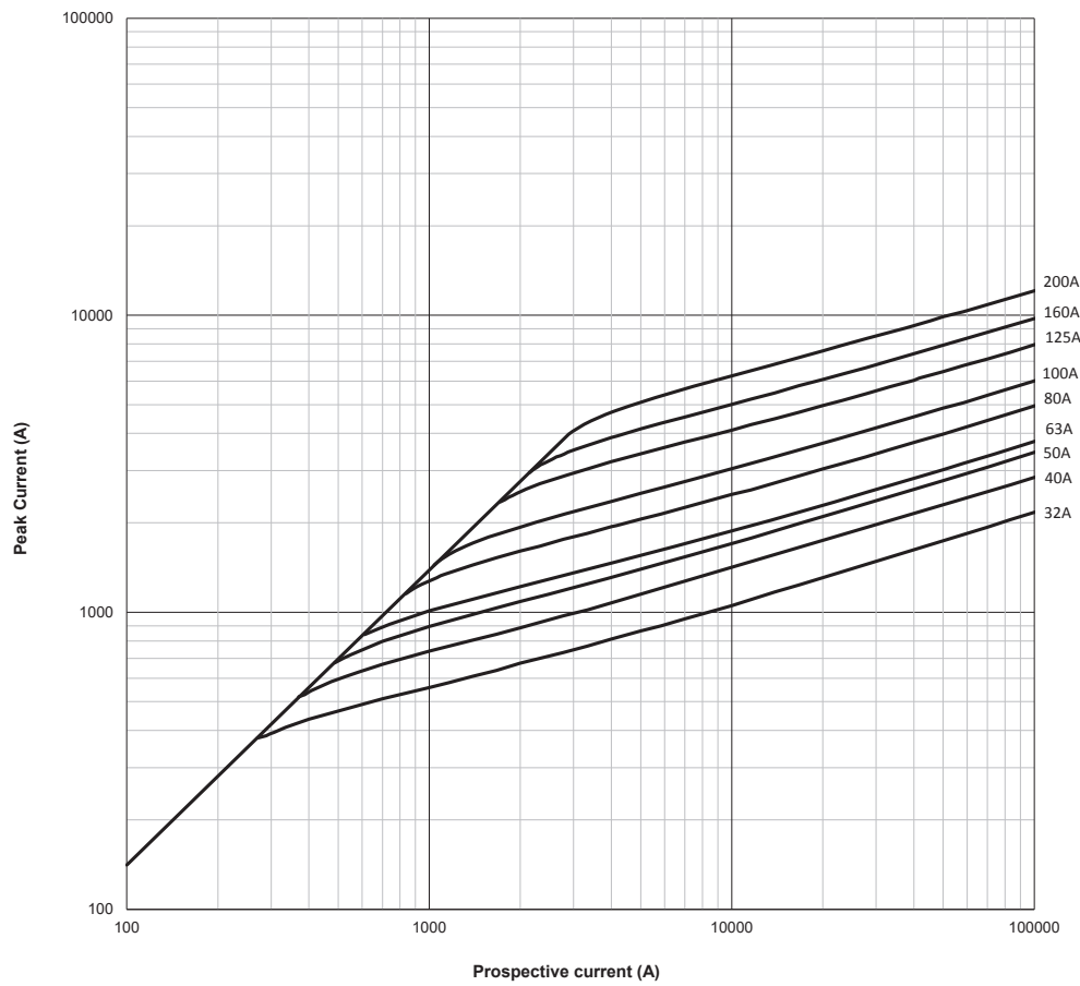
Cut-off peak current characteristic
