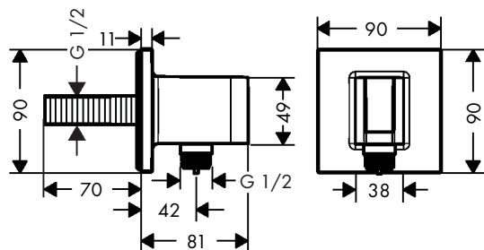
AXOR FixFit Porter Square 36734XX0
