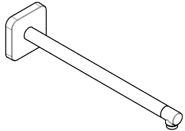
AXOR ShowerSolutions 390 mm softsquare 26967XX0 / 26967XX7
