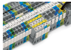
Insulation stop (2002-171) and protective warning marker (2002-115)
