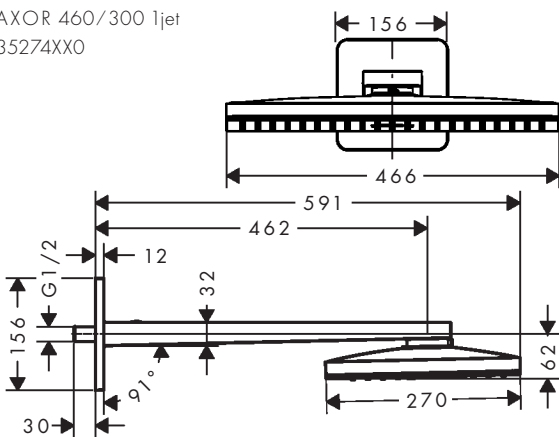
AXOR 460/300 ljet 35278XX0/35274XX0
