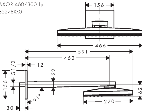
AXOR 460/300 ljet 35274XX0
