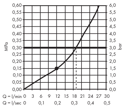
AXOR 460/300 ljet 35278XX0/35274XX0
