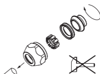
Compression fitting MKV-M
