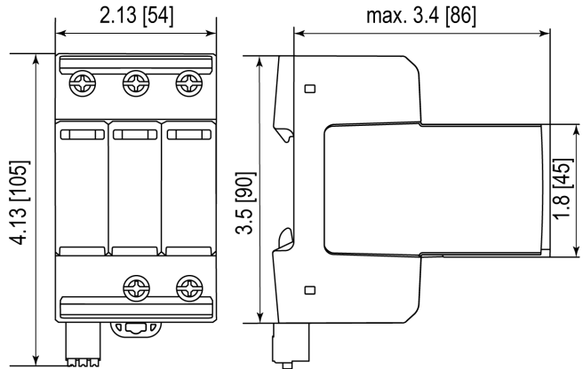
SPHT12-275/3-AX
