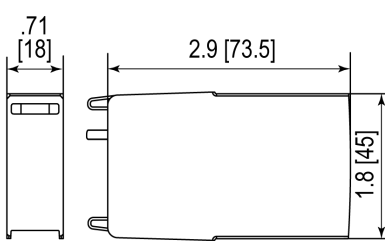
SPHT12-275, SPHT12-305/NPE
