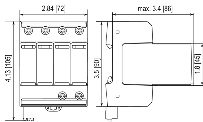
SPHT12-275/3+NPE-AX
