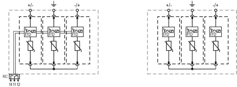
SPHT12-275/3-AX
