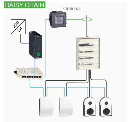
This topology is not recommended since it does not ensure optimum continuity of service
