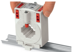
Mounting on DIN-rail via 855-9900 DIN-Rail Adapter
