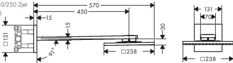
AXOR 300/300 2jet 35318XX0
