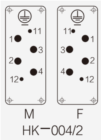
Pin assignment
