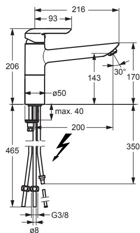
HANSAVANTIS 5249 1177
