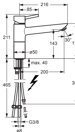
HANSAVANTIS 5249 1173
