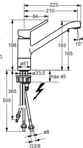
HANSAVANTIS 5249 1177
