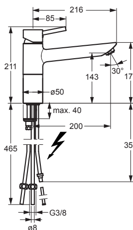
HANSAVANTIS 5249 1173
