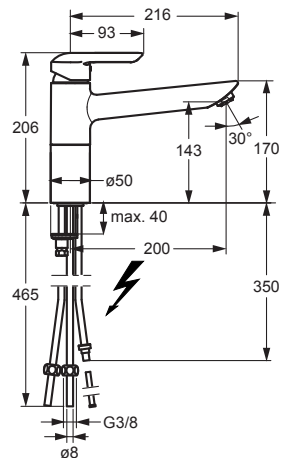
HANSAVANTIS 5249 1177
