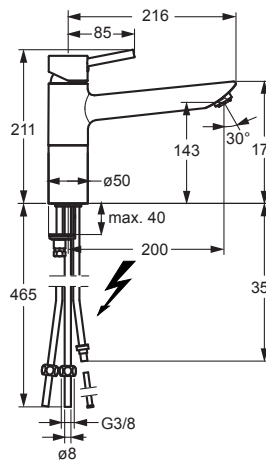
HANSAVANTIS 5249 1173
