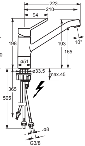
HANSAVANTIS 5249 1177
