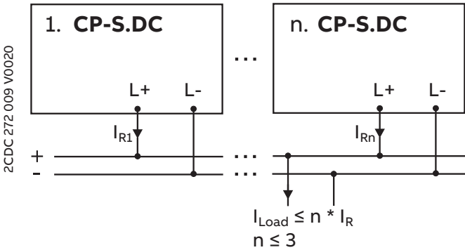
Fig. IV Parallel operation, increased power
