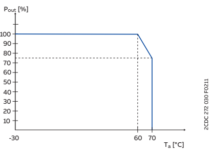
Fig. 5 Derating
