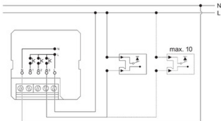
Electronic signal insert with push-button
