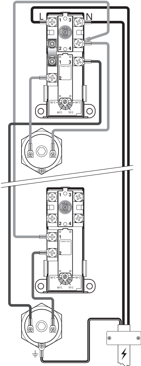
Electrical connection, diagram 4.5+4.5 kW
