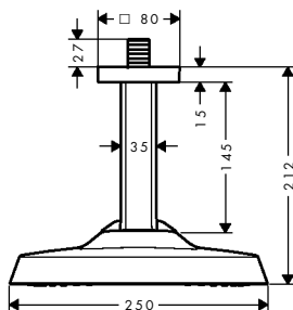
AXOR ShowerSphere 250 / 160 mm 1jet EcoSmart+ 39771XX0
