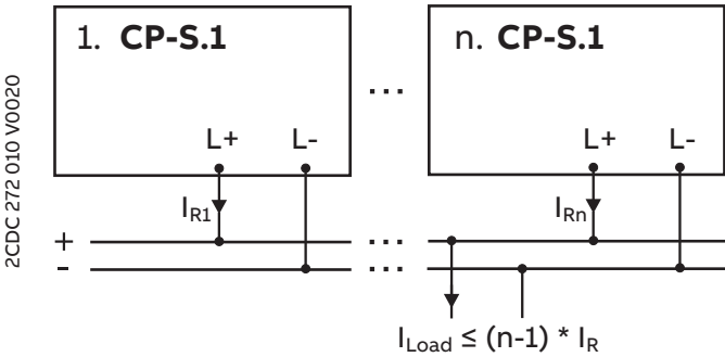
Fig. V Parallel operation, redundancy
