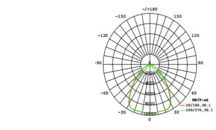
Lens adjust to 80deg
