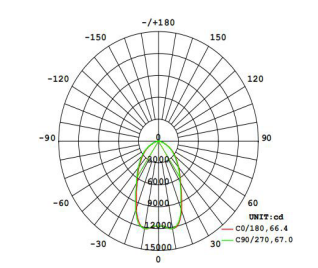
Lens adjust to 60deg
