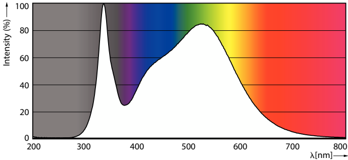
Spectral Power Distribution Colour - CorePro LEDtube 1500mm UO 25.9W 840 T8
