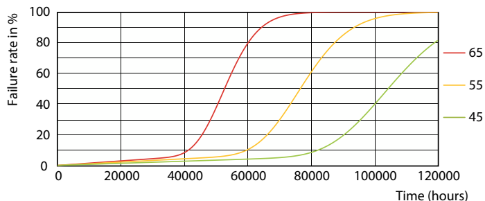
LEDtube-100K-4565-FailureRate-LED
