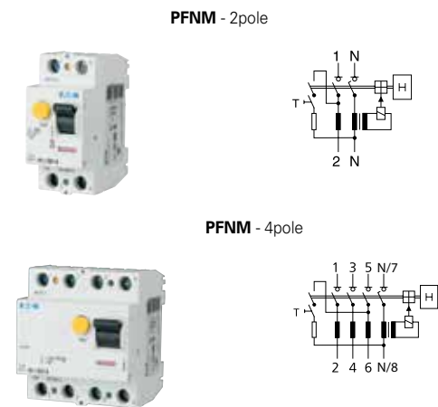
Fig. 35 RCCB without overload protection, a compact device for installation onto DIN rail
