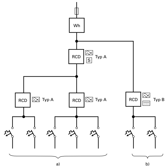
Fig. 85 Example of correct coordination of RCD, type A and B
