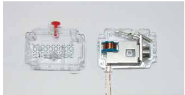
Fig. 9 Trip relay with permanent magnet (PMR)
