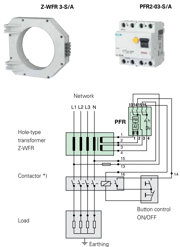
Fig. 36 RCCB with indirect switching with transformer up to 400 A, connection with remote control
