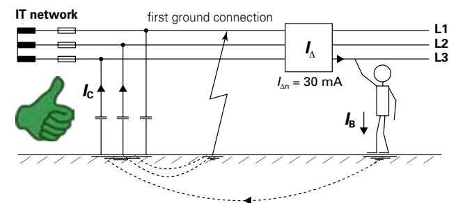
Fig. 57 Correct use of sensitive RCD in an IT network
