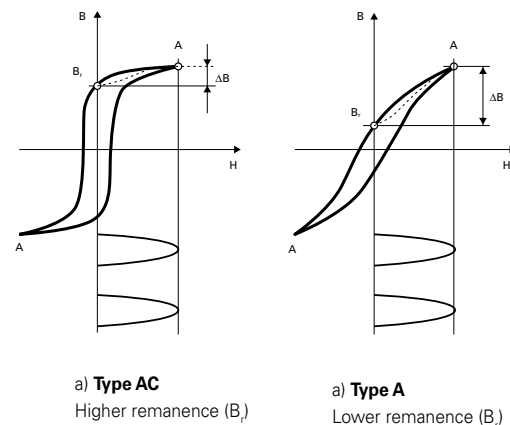
B – magnetic induction [T] H – magnetomotive force [Am -1 ] A – working point for alternate current
