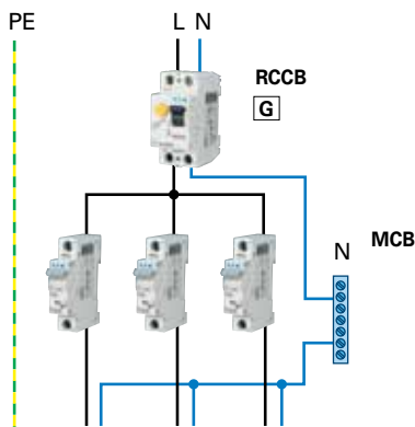
Fig. 77 Grouping of circuits behind RCD
