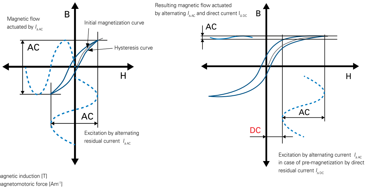
Fig. 26 Impact of direct residual current on core magnetization of summation transformer type A
