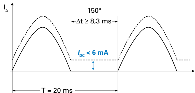
Fig. 25 Definition of pulsating direct component current (6 mA for type A)
