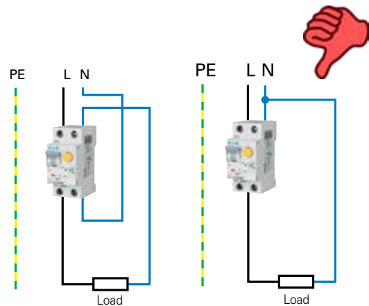
Fig. 95 Incorrect connection of neutral conductor
