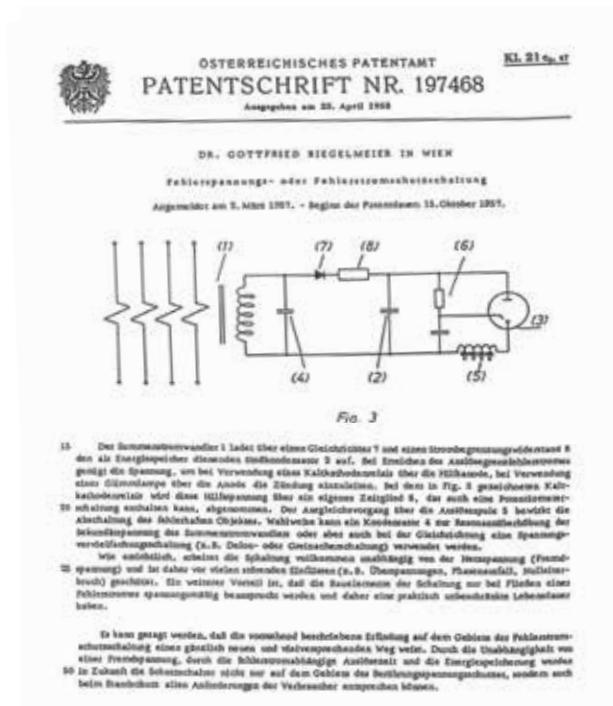
Fig. 3 Patent for residual current device with capacitor as an accumulator, Dr. Gottfried Biegelmeier, Austria, 1957
