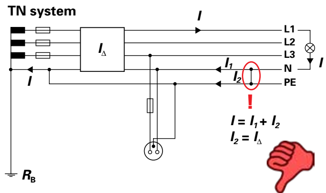
Fig. 91 Impermissible connected PE and N conductors after the RCD
