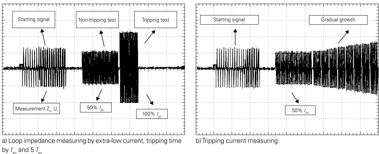
Fig. 73 Examples of passage of measuring currents of a combined device
