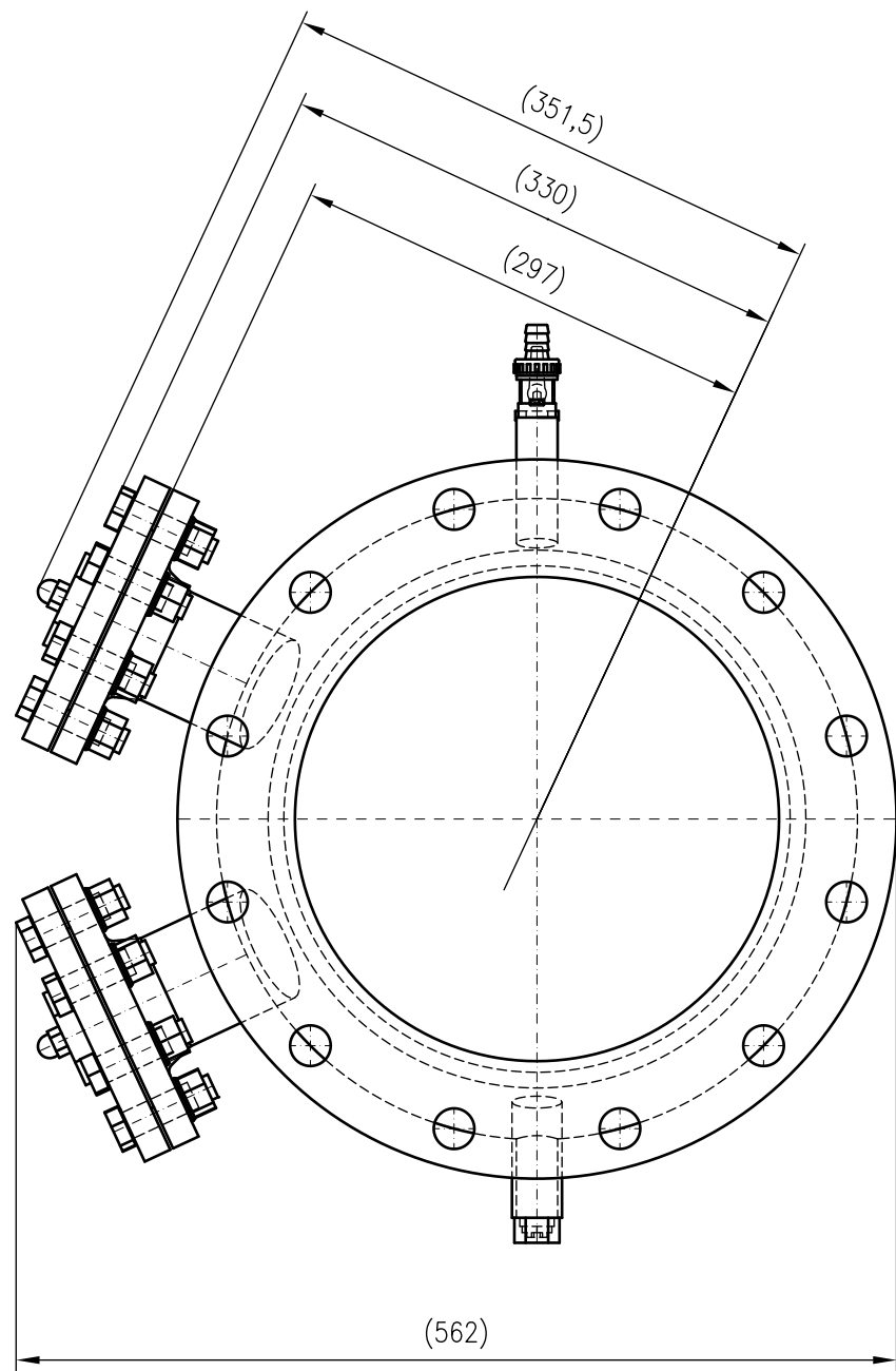
Side view
