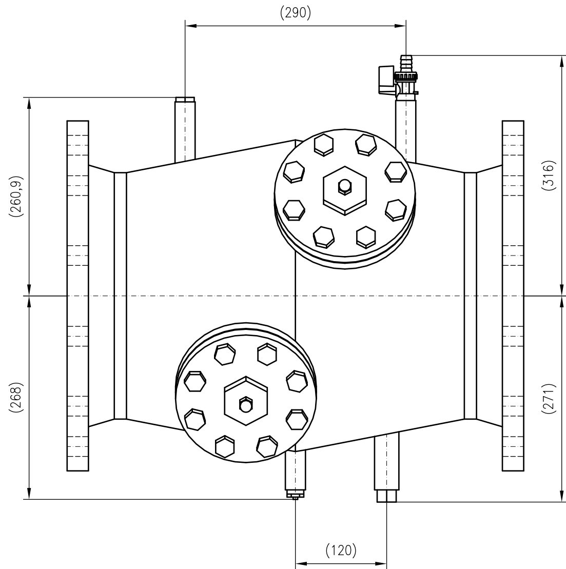
Front view
