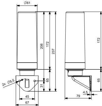
Wall mounting SLC-FW-RYG
