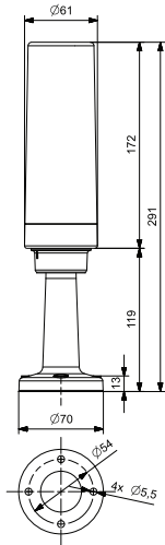
Standard base SLC-100-RYG
