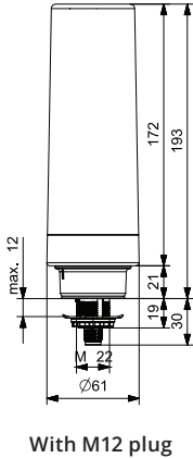
M22 hole mounting SLC-M22-RYG
