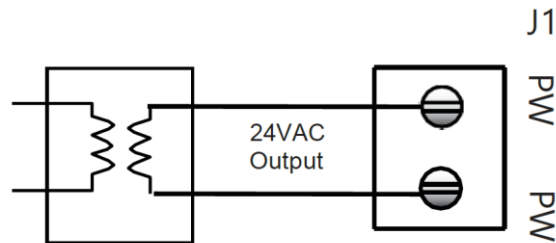
Figure 1-5 Connecting Power to MATRIX Series Area Controller
