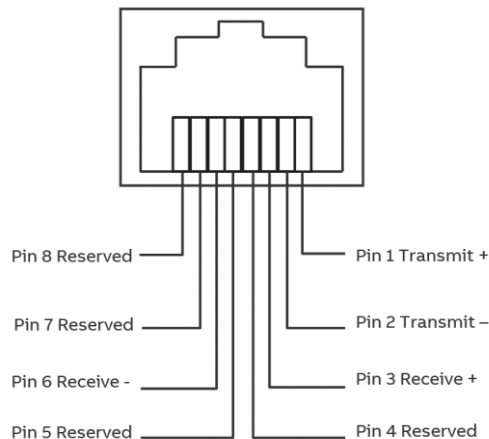
Figure 1-7 Standard Ethernet Connection Pinout
