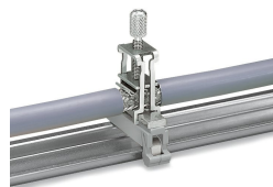
Carrier with grounding foot* (790-113), 45 mm long, busbar 90° to the DIN-rail *for all shield clamping saddle sizes
