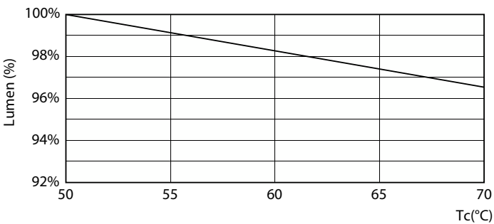
Lumen Maintenance Diagram - LEDtube Connected IA 1200mm 15.6W865 T8
