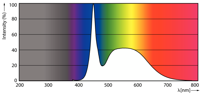
Spectral Power Distribution Colour - LEDtube Connected IA 1200mm 15.6W865 T8
