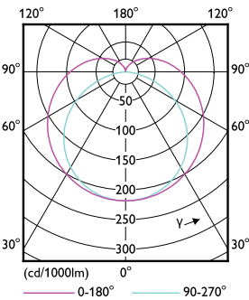
Light Distribution Diagram - LEDtube Connected IA 1200mm 15.6W865 T8
