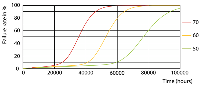
LEDtube-75K-5070-FailureRate-LED
