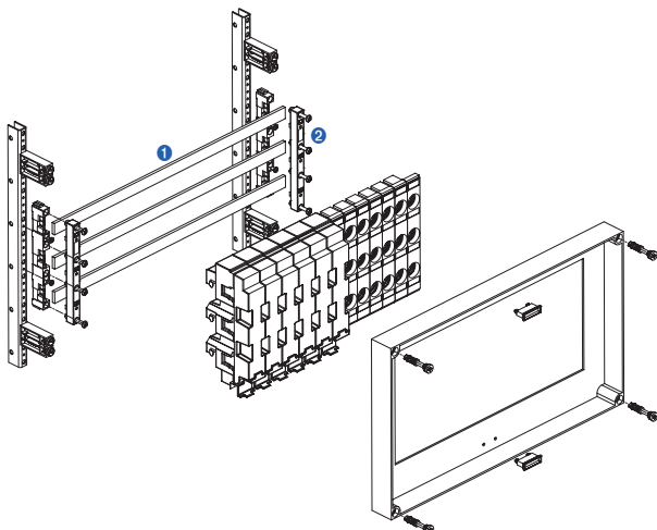
Fig. 3: Busbar-mounted D fuse base, 3 poles, mounted on busbar support. Center-to-center distance between the phases is 60 mm, with Cu busbar system 20x5 or 30x10 mm 1) Busbar system 2) Rail support
