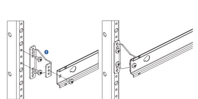
Fig. 4/5: Principle of DIN support rails combined with a set-up bracket and cover plate as a hood 1) Set-up bracket
