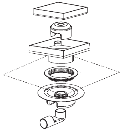
RainDrain Spot Tile 56112800
