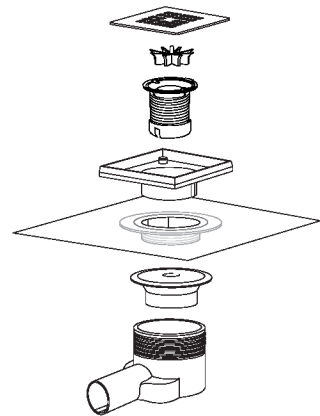
Raindrain Point 56246800 / 56248800
