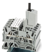
Testing tap (Item No. 2009-182) for tool-free connection of test cables up to 2.5 mm 2 (12 AWG) – compatible with 2000 to 2016 Series
