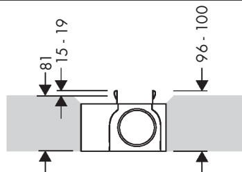
Original standard installation
