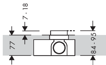
Match/Complete installation set flat Installation
