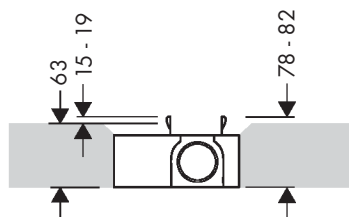
Original flat Installation
