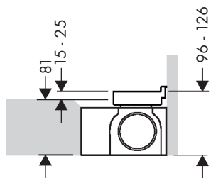
Minimalistic standard installation
