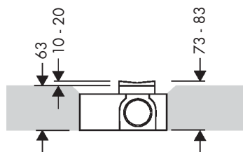
Flex flat Installation
