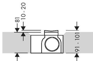
Flex standard installation
