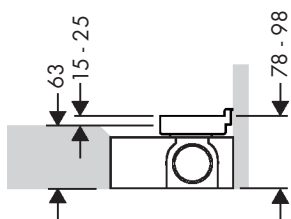
Minimalistic flat Installation
