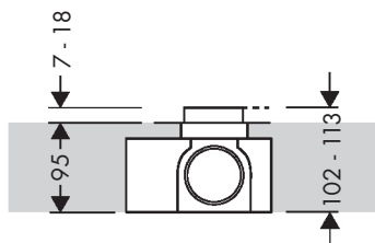
Match/Complete installation set standard installation
