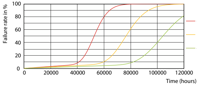
LEDtube_100K_4060_FailureRate-LED
