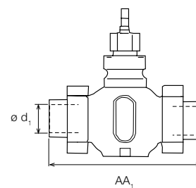
Internal thread connection
