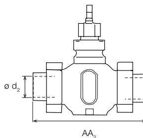
Soldering Type Connection
