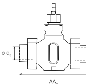
Welded Type Connection
