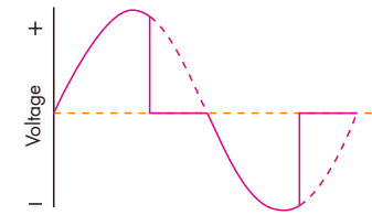
Reverse-phase control dimmer
