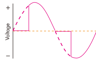
Forward-phase control dimmer(TRIAC)
