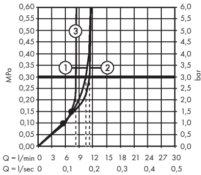
AXOR ShowerSphere 370/220 2jet 39745XX0
