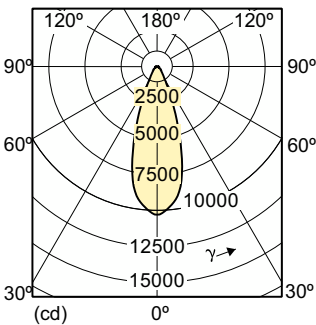
Light Distribution Diagram - MC CDM-R Elite 70W/930 E27 PAR30L 40D
