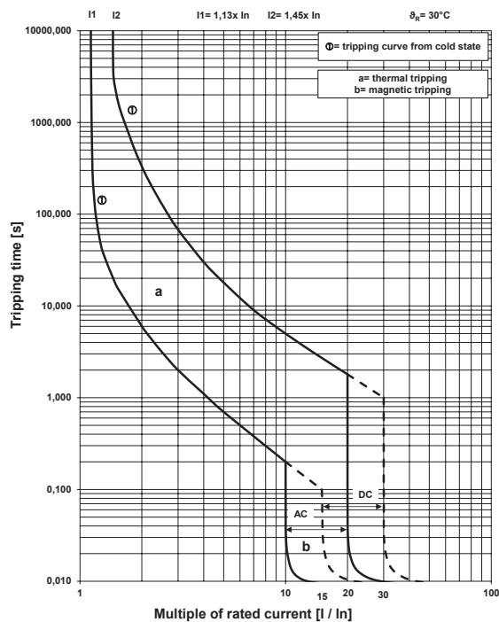
ABB MCB Type S200MT - D Tripping Characteristic 60898-1
