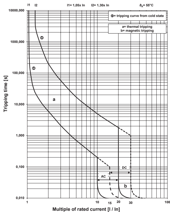
ABB MCB Type S200MT - D Tripping Characteristic 60947-2
