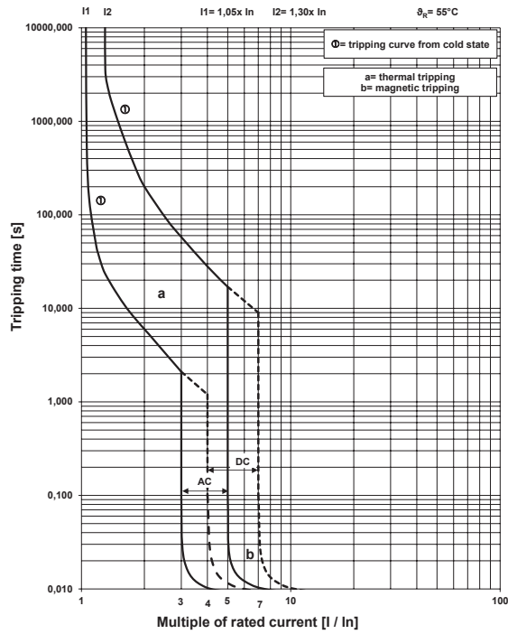
ABB MCB Type S200MT - B Tripping Characteristic 60947-2
