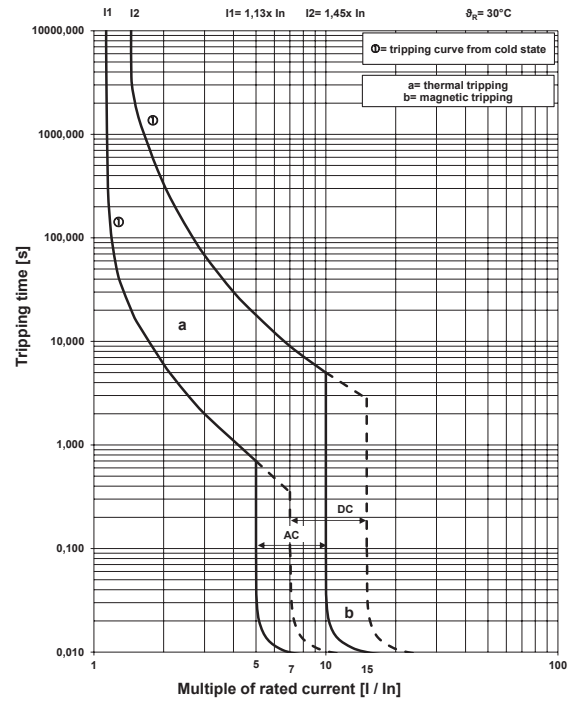
ABB MCB Type S200MT - C Tripping Characteristic 60898-1
