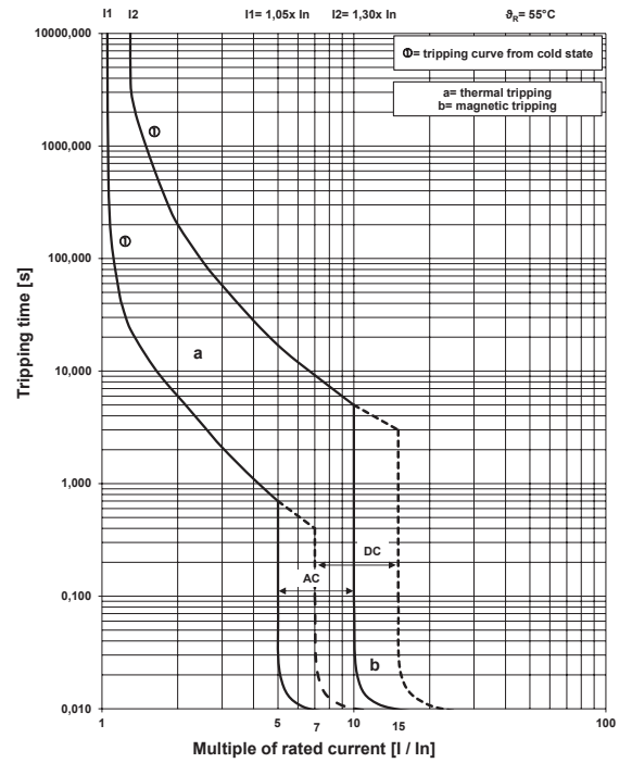
ABB MCB Type S200MT - C Tripping Characteristic 60947-2
