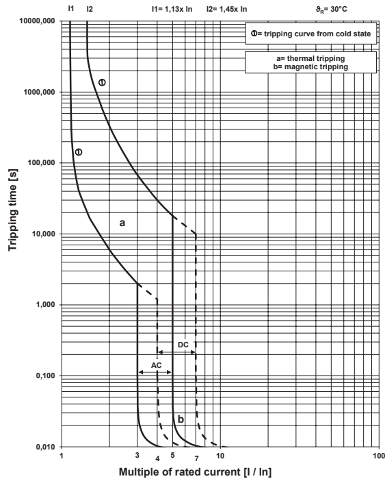
ABB MCB Type S200MT - B Tripping Characteristic 60898-1
