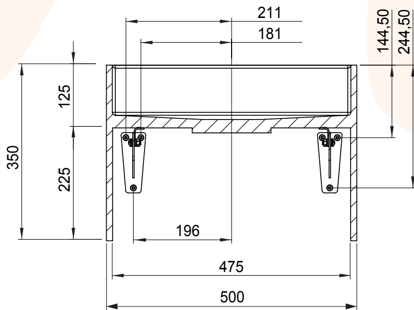
SECTION B-B
