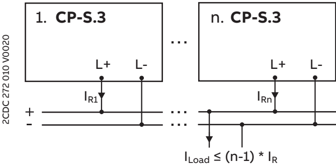
Fig. V Parallel operation, redundancy
