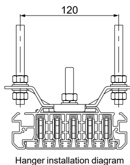
Hanger installation diagram
