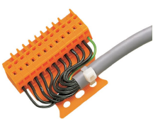
Male connector with strain relief plate
