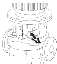
Fig. 17: Vahehargi kohaleasetamine
