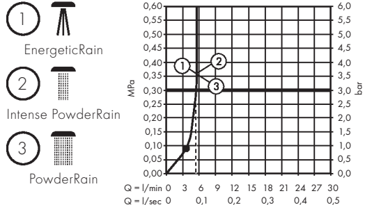
AXOR ShowerSolutions 130 3jet EcoSmart+
