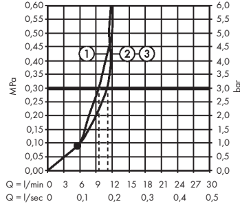
AXOR ShowerSolutions 130 3jet EcoSmart+
